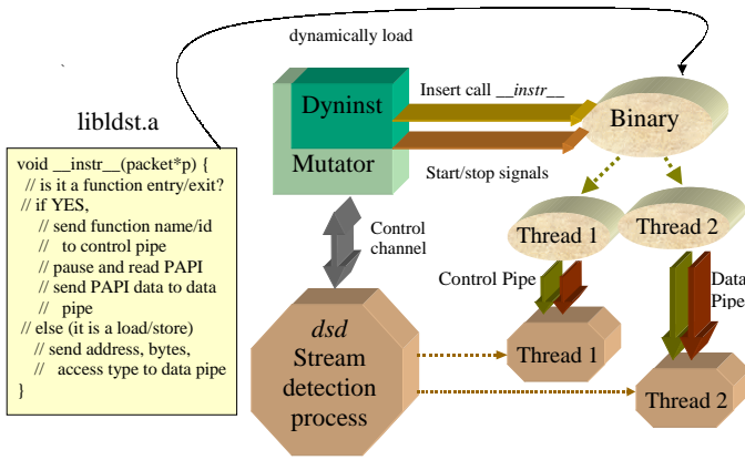
Figure 3: Stream detection framework
