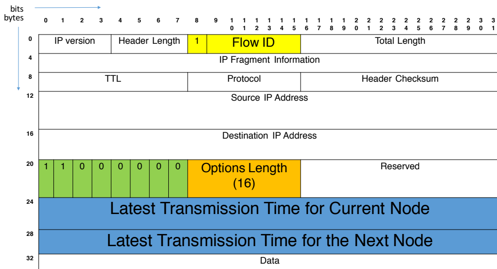
Figure 2 Message Header
